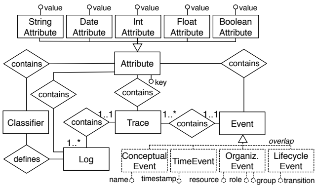
Fig. 10 E-R diagram capturing a portion of the XES meta-model; the dashed part is reported for clarity, but is concretely realized in XES through the notion of extension and corresponding required attributes for the events.
