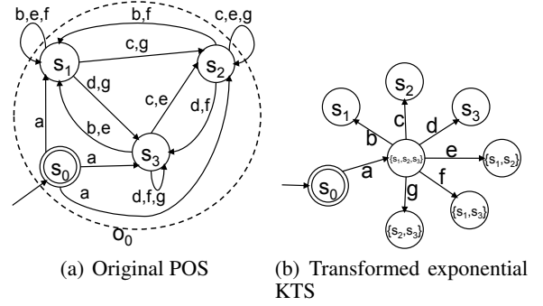
Figure 3: Example of Worst Case Transformation.
